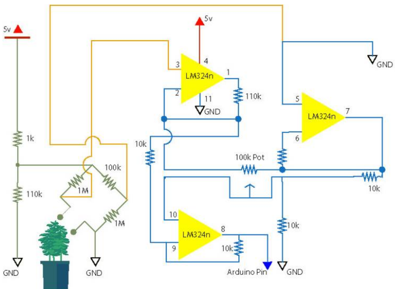
Galvanic sensor
