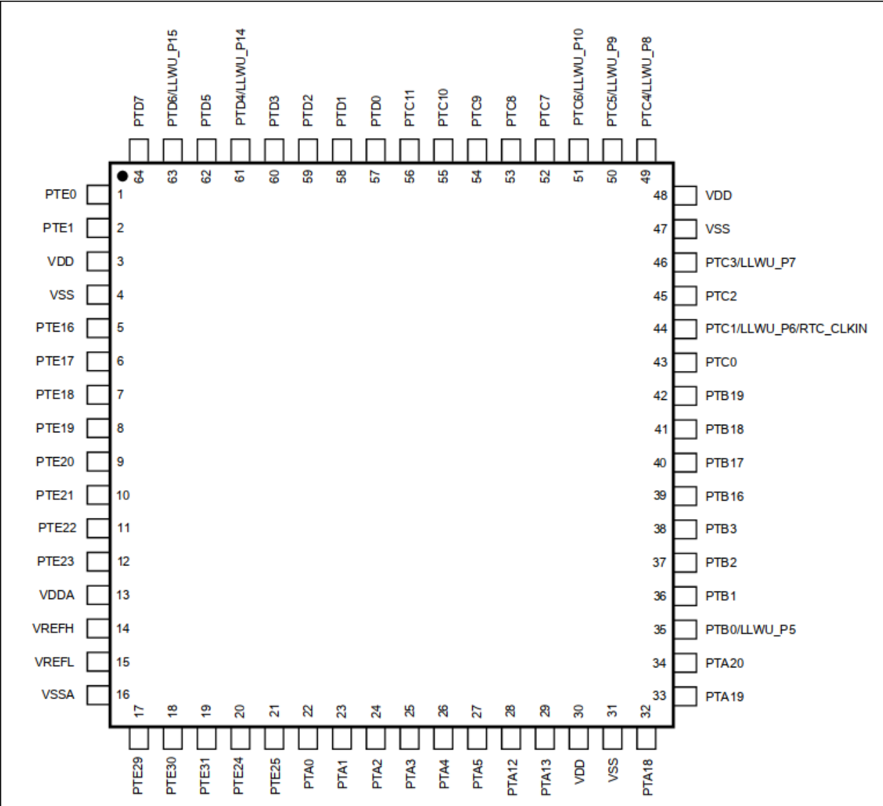
Figure 22. KL16 64-pin LQFP pinout diagram
